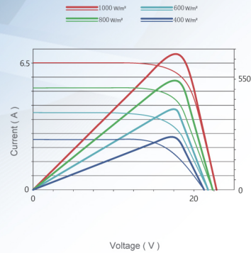
Current-Voltage & Power-Voltage Curves(550W)
